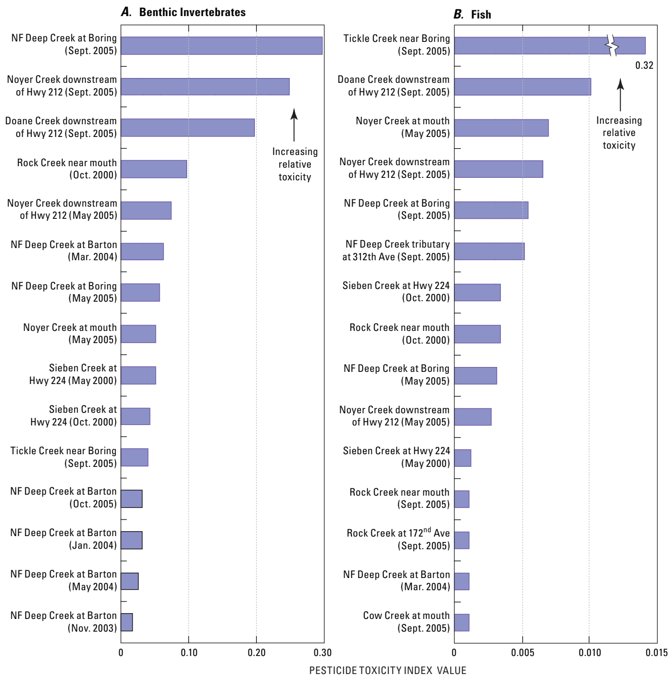
Figure 13. {Graphs showing} highest Pesticide Toxicity Index values for benthic invertebrates and fish for samples collected from the lower Clackamas River basin tributaries, Oregon, 2000–2005.
