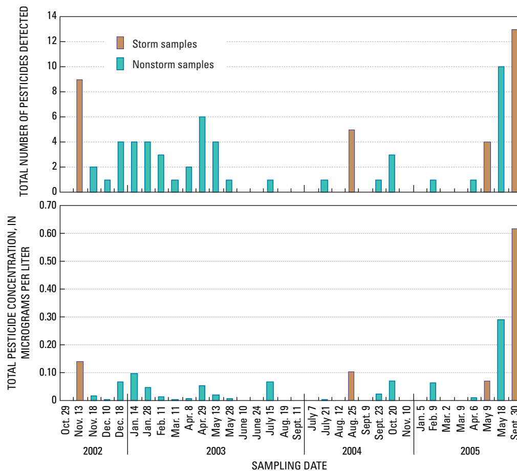
Figure 10. {Graphs showing} total number of pesticides detected and total pesticide concentrations for storm and nonstorm samples of source water collected from the study water-treatment plant on the lower Clackamas River, Oregon, 2002–2005.
