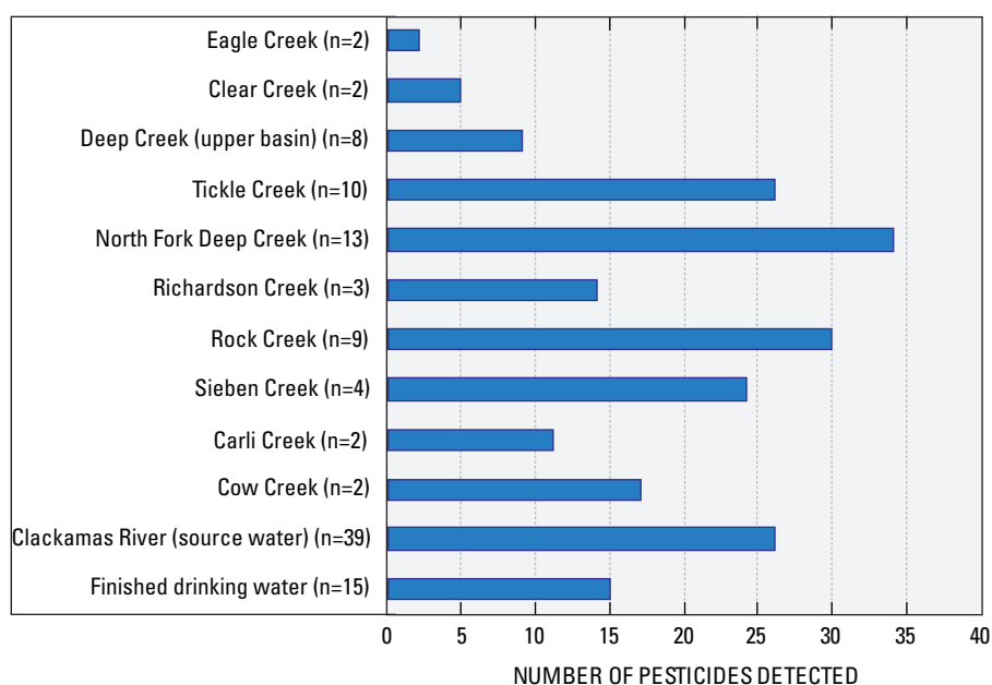
Figure 7. {Graph showing} number of pesticide compounds detected in samples collected from the lower Clackamas River basin tributaries and in source and finished drinking water from the study water-treatment plant on the lower Clackamas River, Oregon, 2000–2005.
