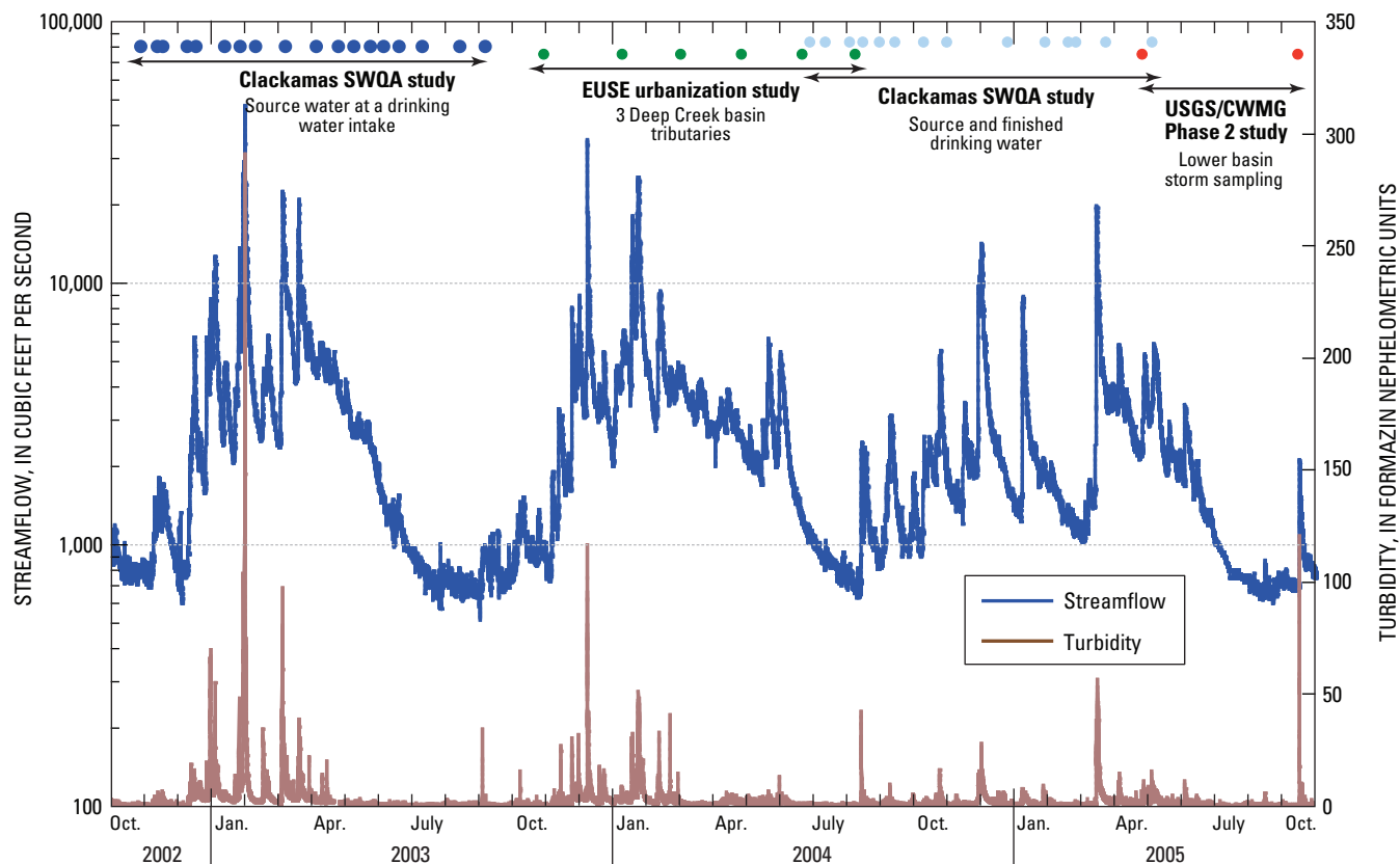
Figure 2. {Graph showing} distribution of data-collection activities and streamflow and turbidity conditions in the lower Clackamas River at Oregon City, Oregon, 2002–2005.
