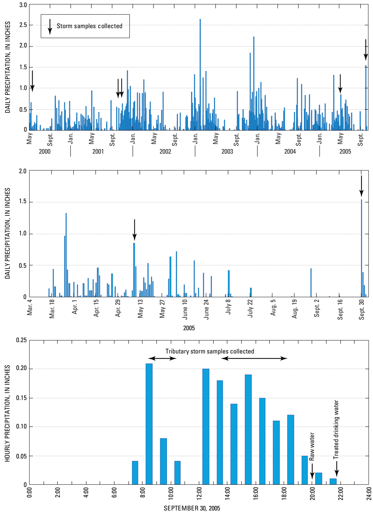
Figure 4. {Graphs showing} daily and hourly precipitation at the Holgate Road rain gage and distribution of storm samples collected in the lower Clackamas River basin, Oregon, 2000–2005.
