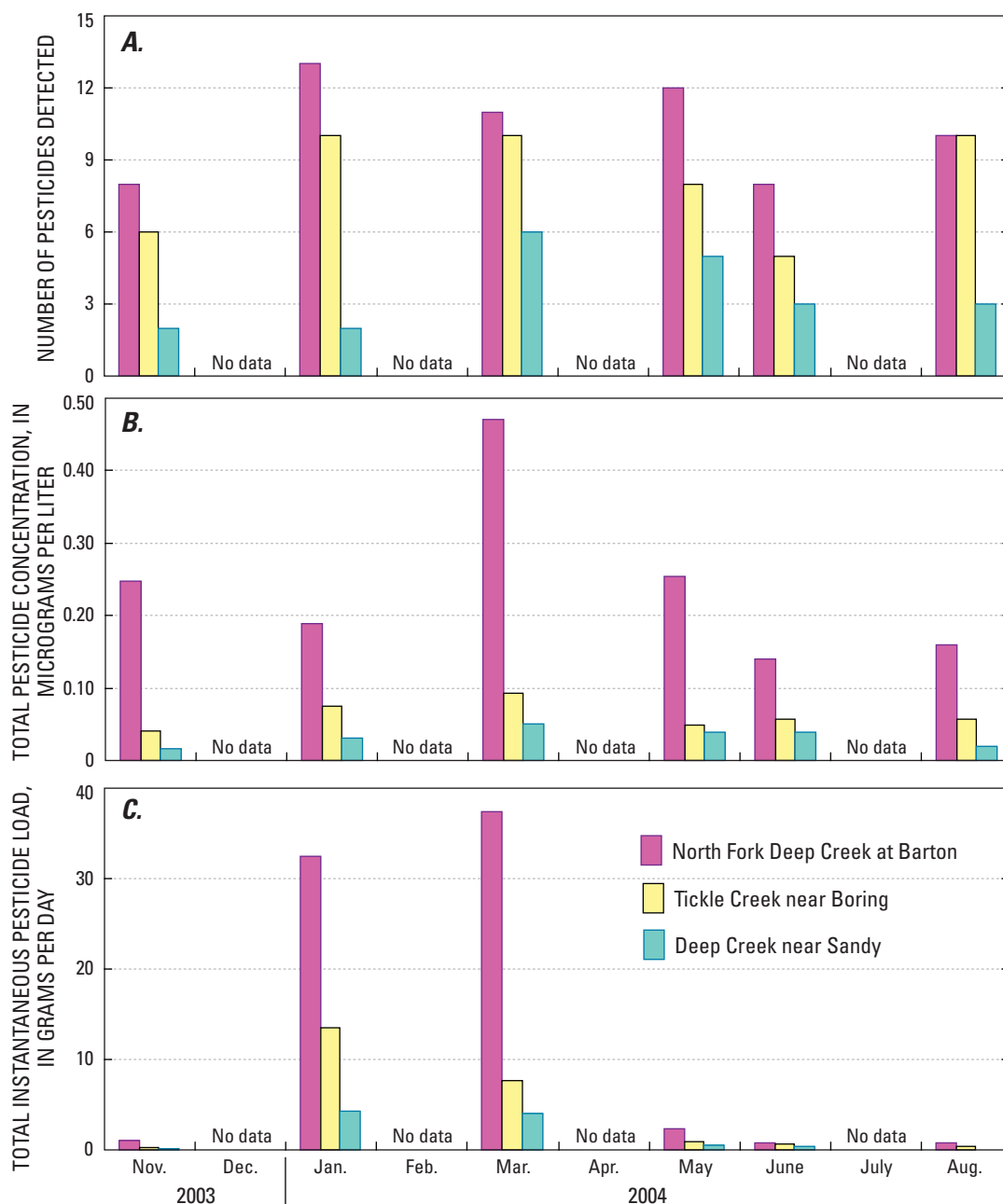
Figure 9. {Graphs showing} number, total concentration, and total instantaneous load of pesticides for samples collected during the EUSE urbanization study from three streams in the Deep Creek basin, Oregon, 2003–2004.
