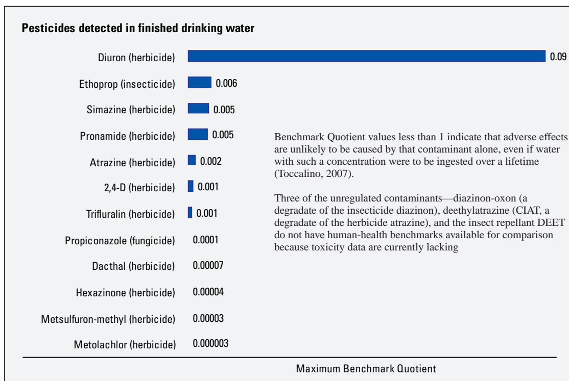
Figure 14. {Graph showing} maximum benchmark quotients for pesticide concentrations in finished drinking-water samples from the study water-treatment plant on the lower Clackamas River, Oregon, 2004–2005.
