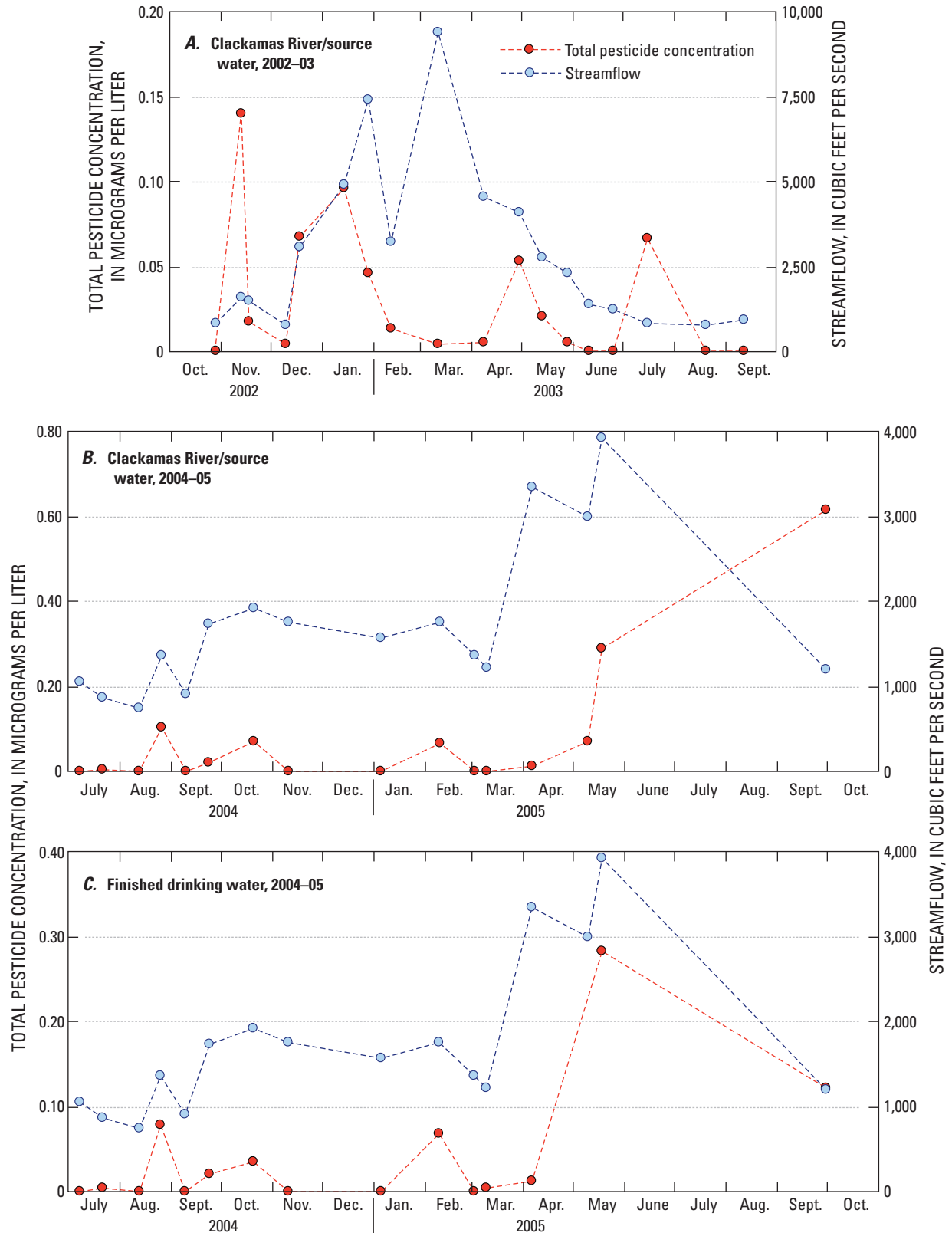
Figure 11. {Graphs showing} total pesticide concentrations in source and finished drinking water samples collected from the study water-treatment plant on the lower Clackamas River, Oregon, 2002–2005.
