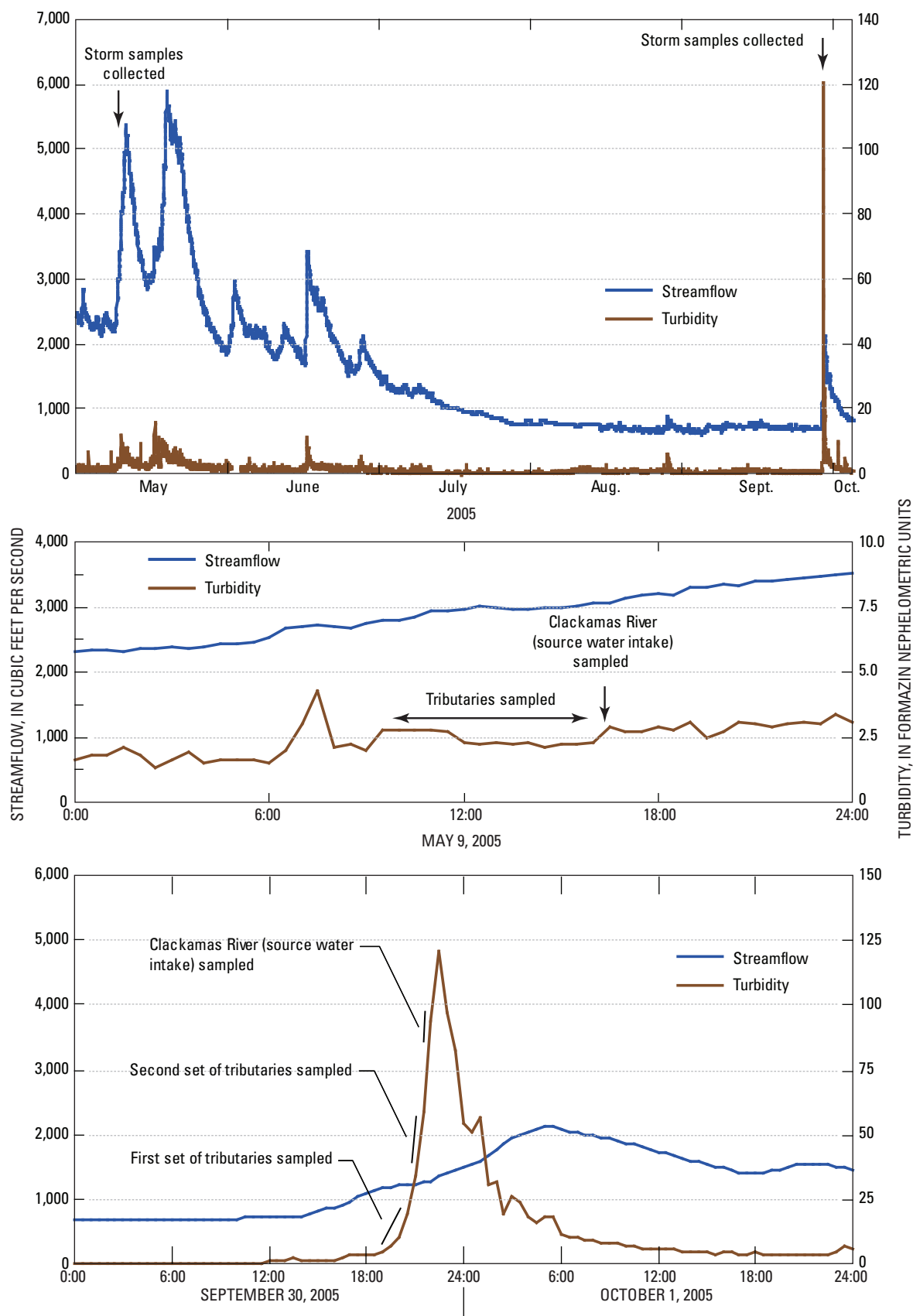
Figure 3. {Graphs showing} streamflow and turbidity conditions in the lower Clackamas River at Oregon City, Oregon (USGS continuous water-quality monitor and streamflow-gaging station 14211010), during the May and September 2005 storm event samplings.
