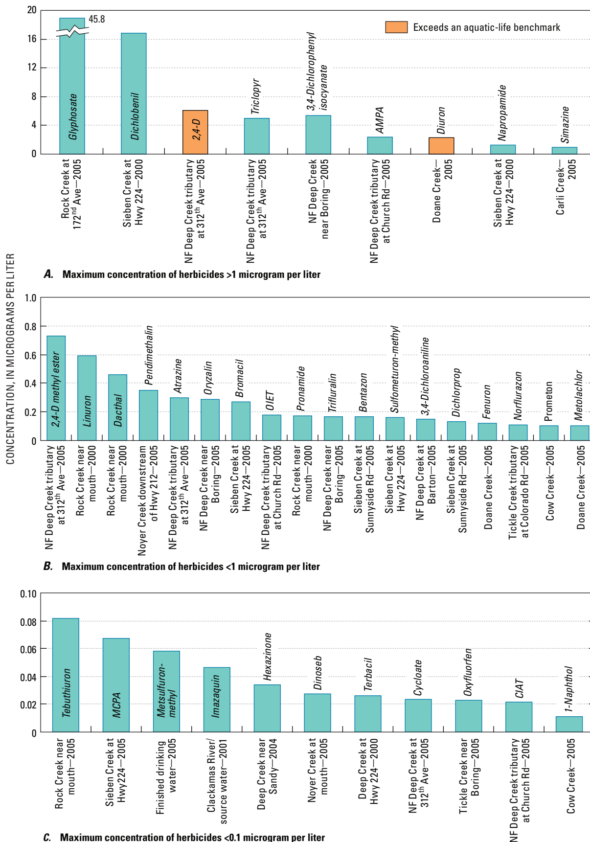
Figure 8. {Graphs showing} maximum concentrations of herbicides, insecticides, and fungicides detected in samples collected from the lower Clackamas River basin, Oregon, 2000–2005.
