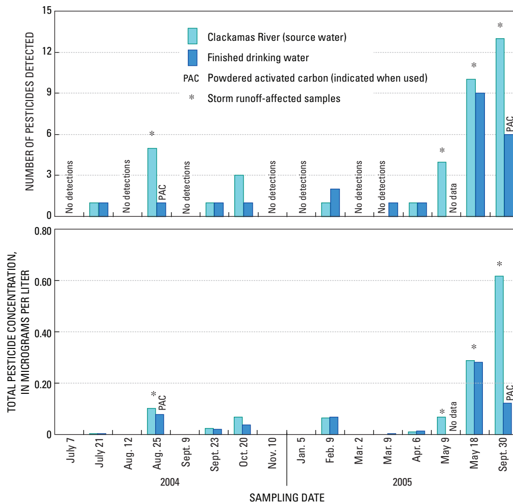
Figure 12. {Graphs showing} number of pesticides detected and total pesticide concentrations in source and finished drinking water samples collected from the study water-treatment plant on the lower Clackamas River, Oregon, 2004–2005.
