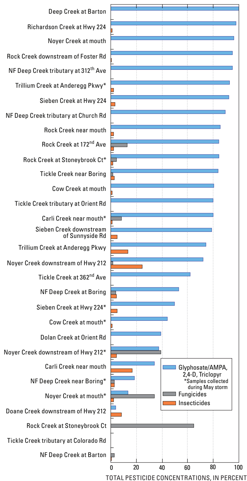
Figure 6. {Graph showing} percentage of total pesticide concentration from the common herbicide products RoundUP™ (glyphosate and its degradate AMPA) and Crossbow™ (2,4-D and triclopyr), fungicides, and insecticides for storm samples collected from tributaries, May and September 2005. (Samples are sorted by percentage of glyphosate/AMPA, 2,4-D, and triclopyr.)
